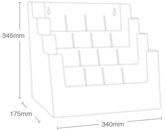
4C330 - supplied with 8 removable CD pocket dividers 8 pocket A5 portrait leaflet holder Carton quantity 8 Opening dimensions: 330 x 32mm
