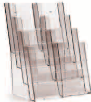
4C230 - supplied with 4 removable CD pocket dividers 4 pocket A4 portrait leaflet holder Carton quantity 8 Opening dimensions: 230 x 32mm
